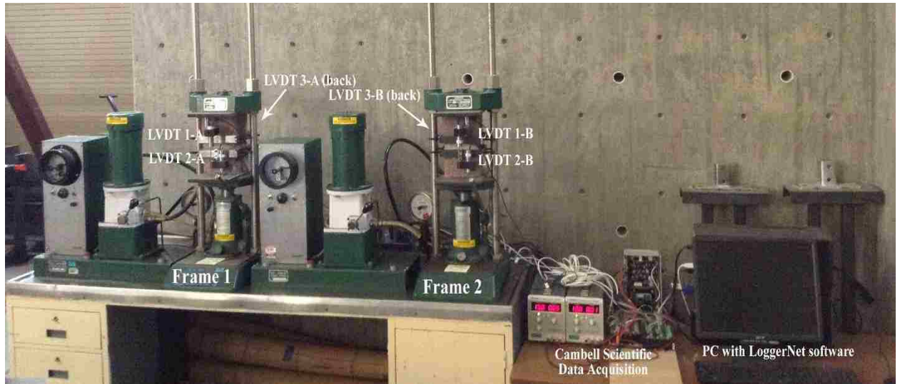
Figure 3.35. SCEB 7 prisms placed on the Carver Press and displacement measured using the Campbell Scientific Data Acquisition.
