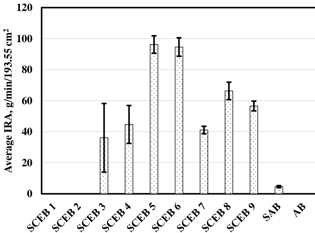
Figure 4. 25. Initial rate of absorption results plotted.
