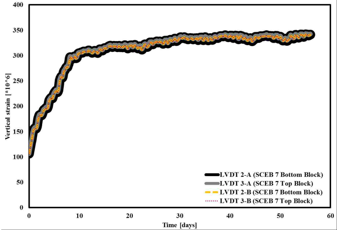
Figure 4. 37. Vertical Elastic Strain for SCEB 7.
